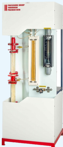
PRESSURE DROP THROUGH PACKED BED
